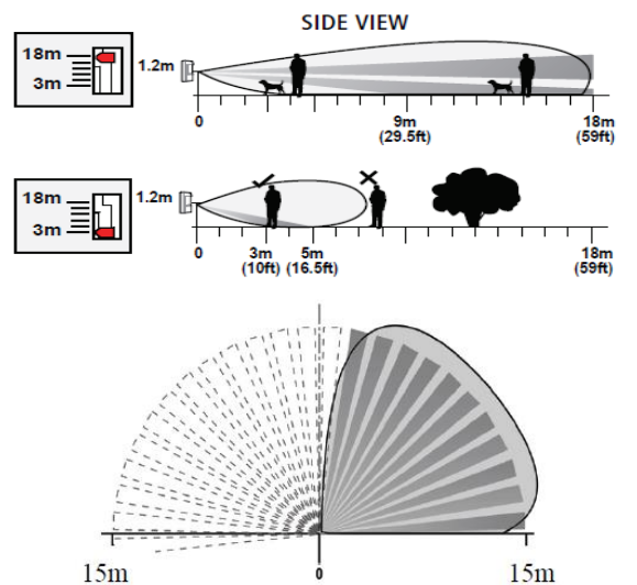
Detection beam direction adjustable between 0° and 180°
