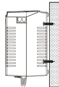
Chart3. Mounting vertically
